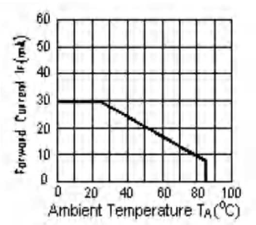
I LED VS TEMP
